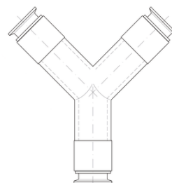
Y-SHAPE
